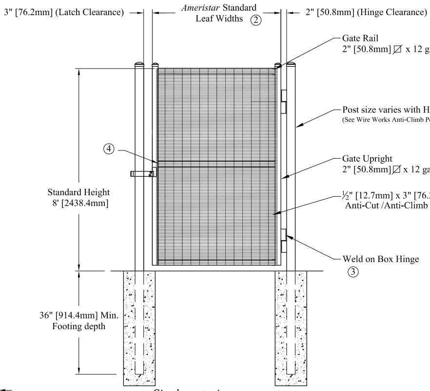
Single gate Arrangement
