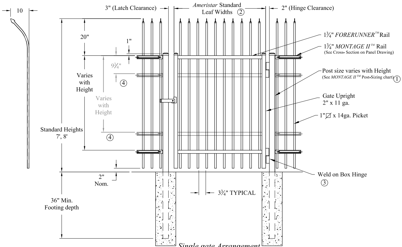
Single gate Arrangement
