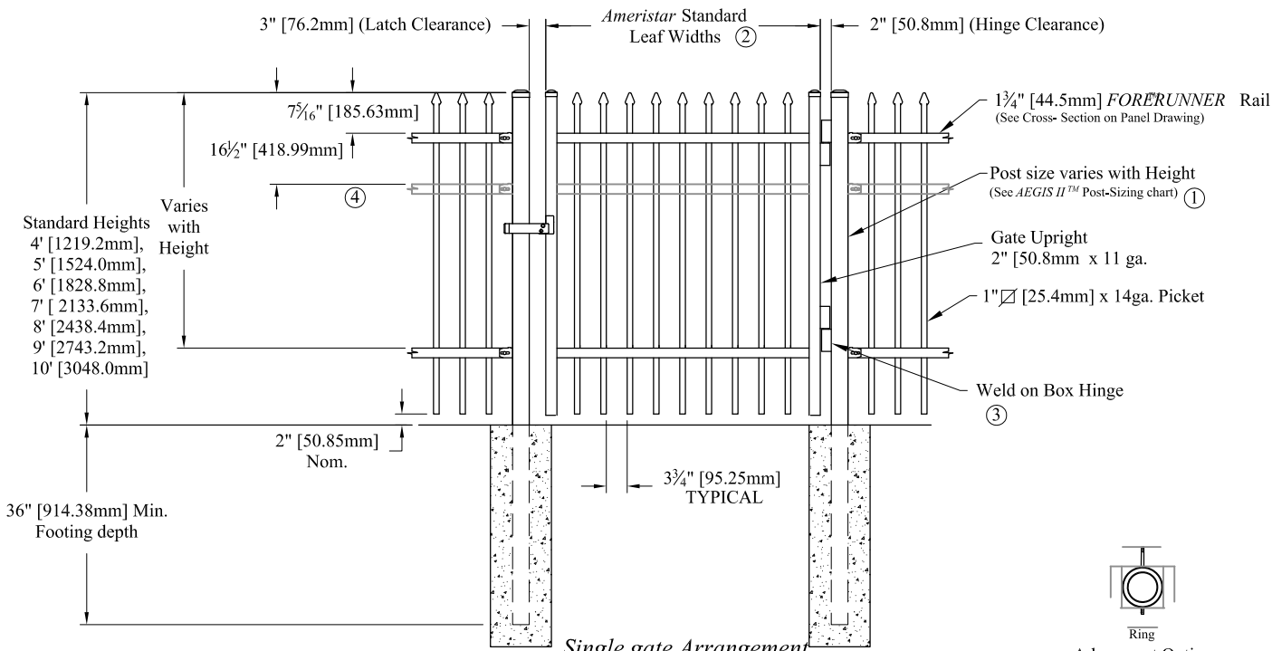
Single gate Arrangement
