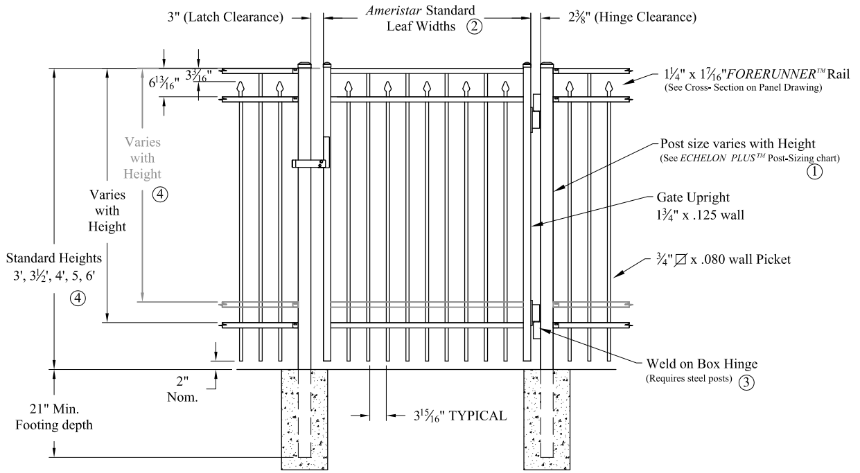
Single gate Arrangement
