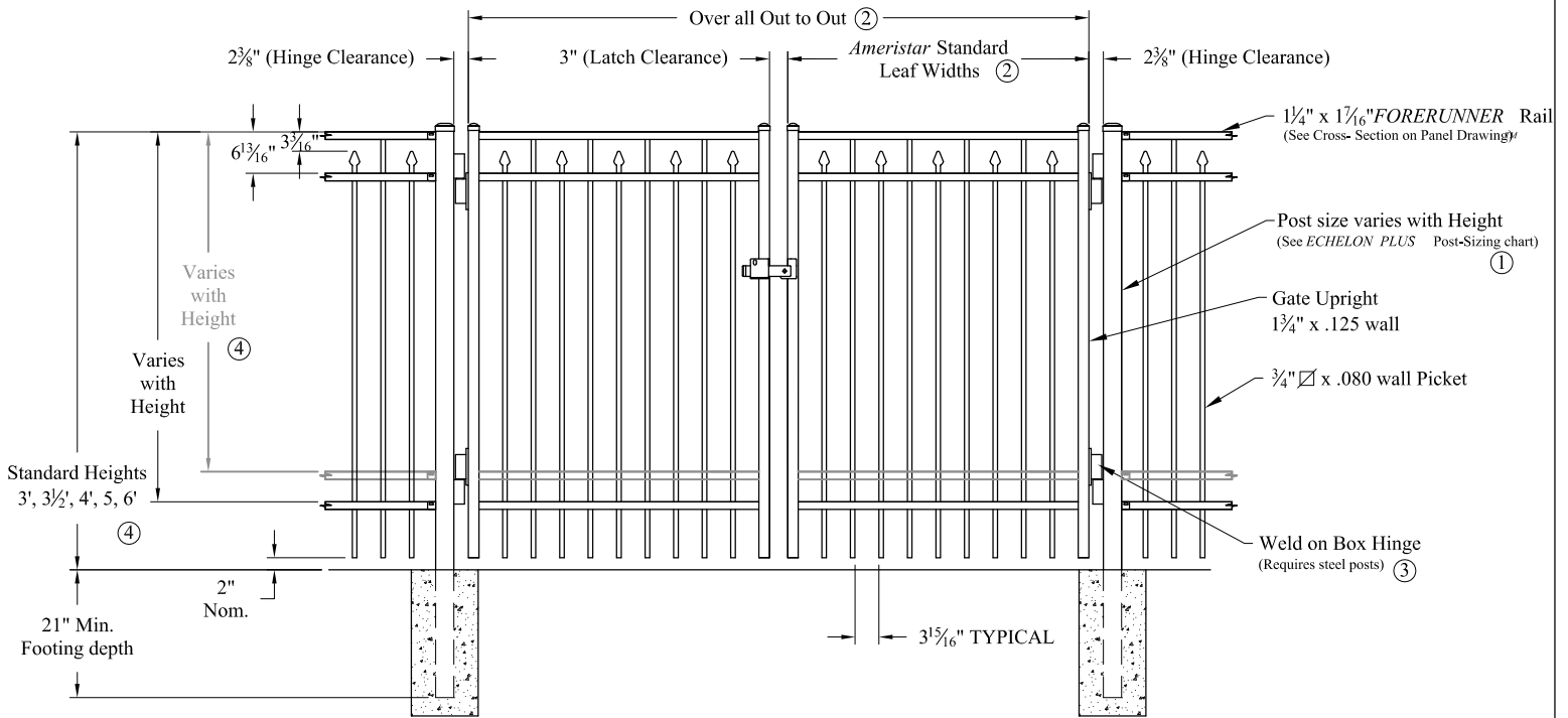
Double gate Arrangement
