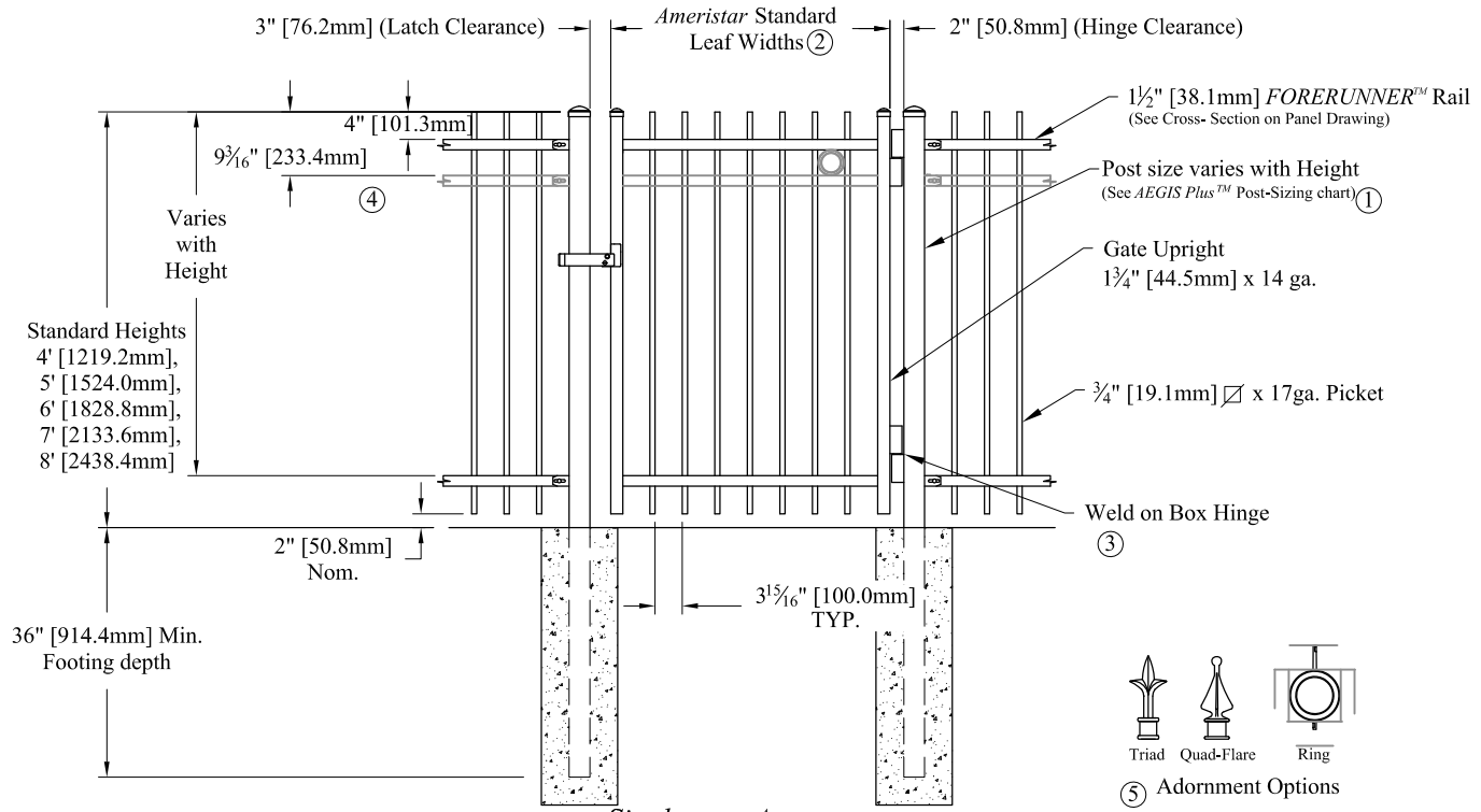
Single gate Arrangement
