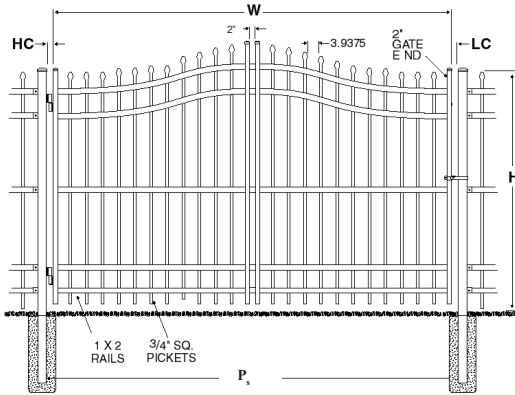
Order 1 Leaf For Single Swing Opening (Available only as single)
