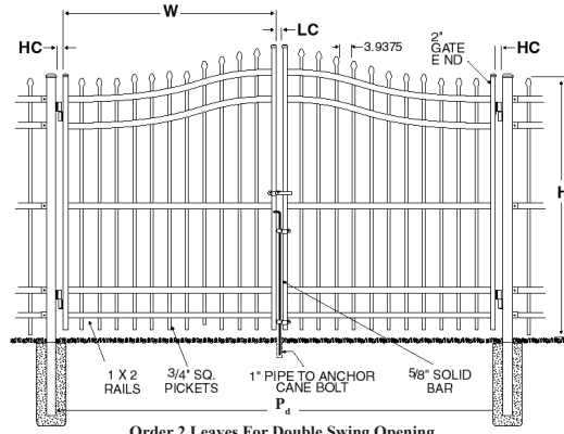
Order 2 Leaves For Double Swing Opening
