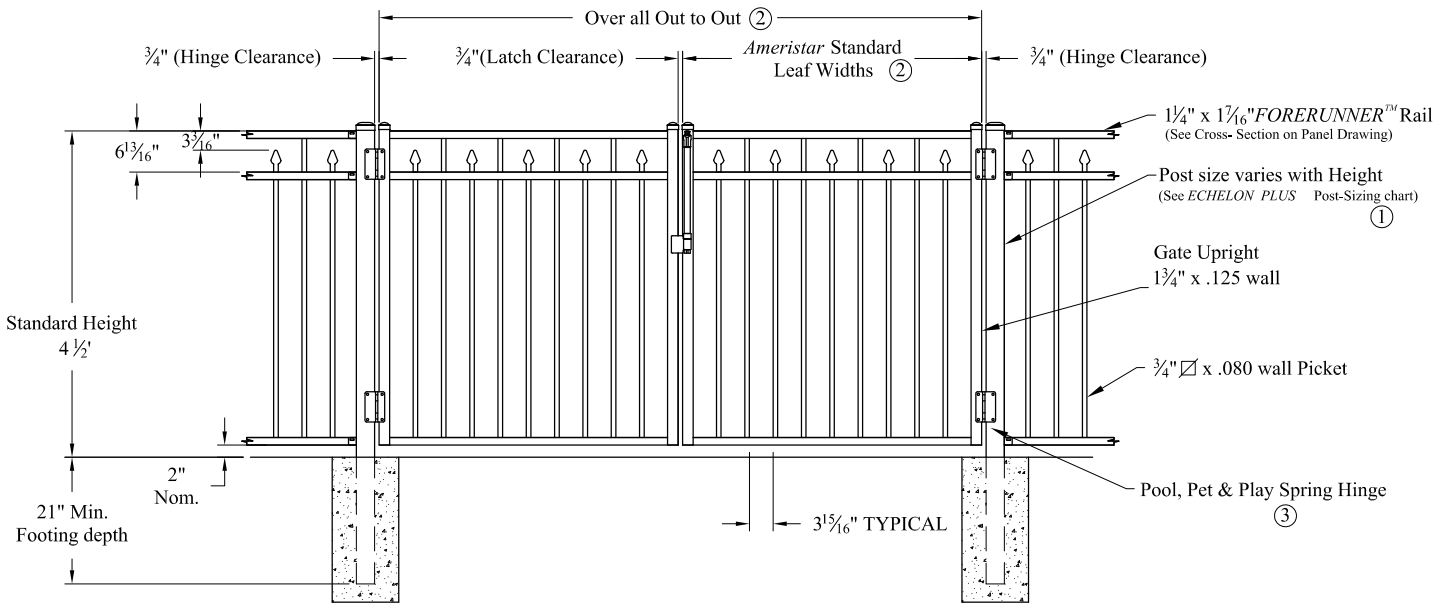
Double gate Arrangement
