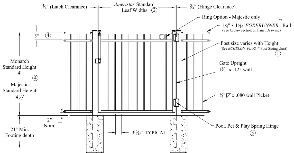
Single gate Arrangement
